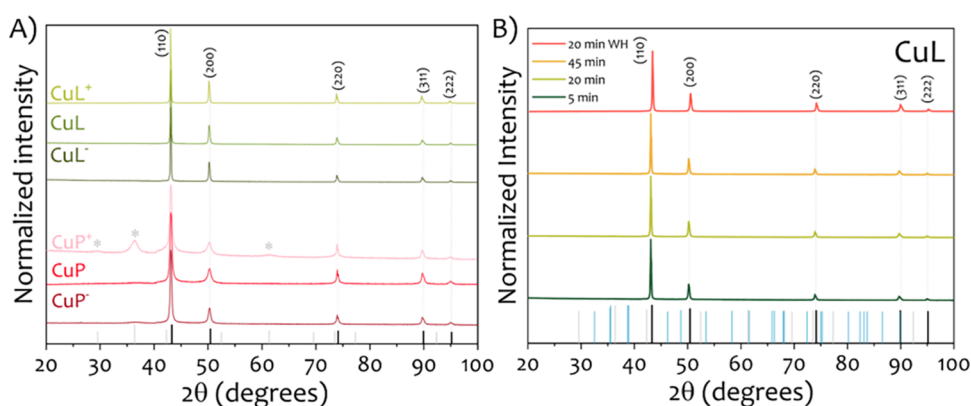
Figure 5. (A) PXRD diffractograms of Cu NPs synthesized with different amounts of both lignin and capping agents. Samples CuL + , CuL, and CuL - correspond to high, standard, and low concentrations of lignin, respectively. Similarly, CuP + , CuP, and CuP - represent high, standard, and low concentrations of PVP. PXRD diffractograms of the samples obtained with different amounts of capping agents, both PVP and lignin. (B) PXRD diffractograms of the samples obtained at different reaction times (5, 20, and 45 min) when lignin is used as capping agent. The sample labeled “20 min WH” corresponds to a synthesis performed without the preheating and homogenization steps, where microwave heating was applied directly until 70 °C was reached and then maintained for 20 min. PXRD patterns for Cu (PDF 00-004-0836), CuO (PDF 00-041-0254), and Cu 2 O (PDF 00-005-0667) are represented in black, blue, and gray, respectively. Symbols * indicate the indexed Cu 2 O diffraction peaks.
