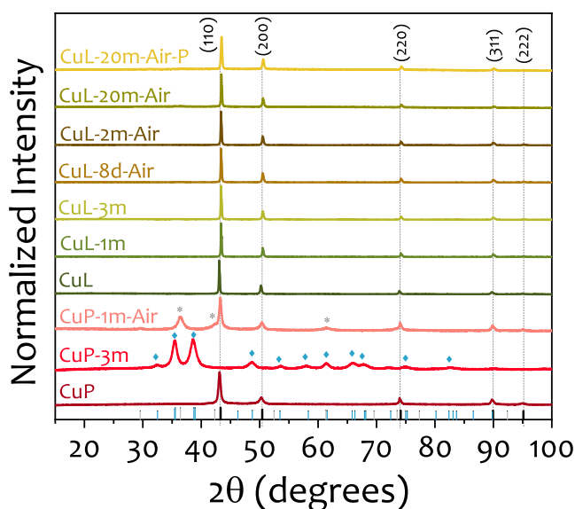
Figure 6. Evolution of the PXRD diffractograms of the samples under different time and storage conditions. PXRD patterns for Cu (PDF 00-004-0836), CuO (PDF 00-041-0254), and Cu 2 O (PDF 00-005-0667) are represented in black, blue, and gray, respectively. Symbols * and ♦ indicate the indexed Cu 2 O and CuO diffraction peaks, respectively. Sample names indicate the storage duration in days (d) or months (m) (e.g., 8d for 8 days, 1m for one month). Samples stored in ethanol carry no additional label; those labeled "Air" were stored as dry powders in ambient conditions; samples marked "P" refer to powders compacted into pellets and stored in air.
